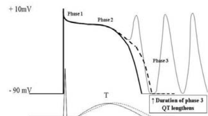
Early Afterdepolarization (EAD) (Effect of Potassium Channel Blockers)
